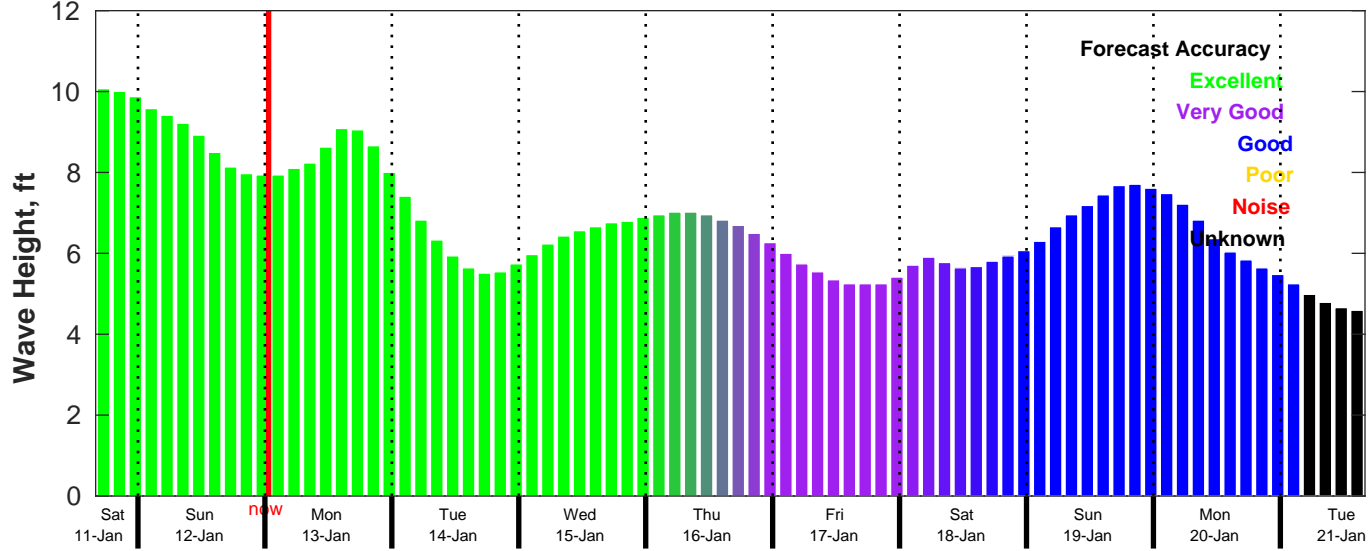
CMEMS Wave Forecast for NDBC 46011 from 11-Jan-2025 16:00:00 to 21-Jan-2025 16:00:00
