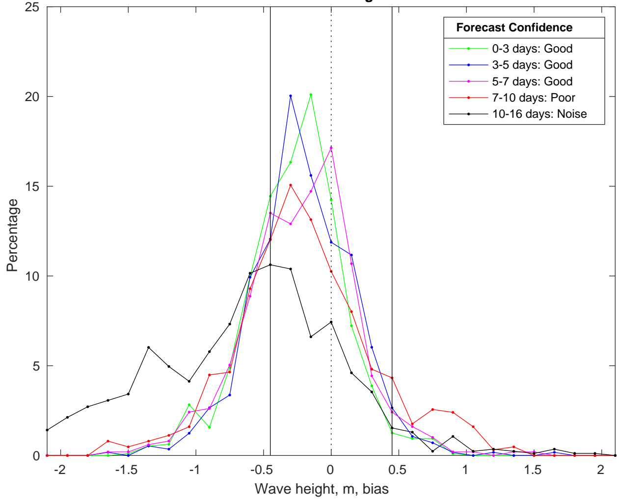
NDBC 46028 vs GFSWaves Bias Histogram: 13-Jan-2025
