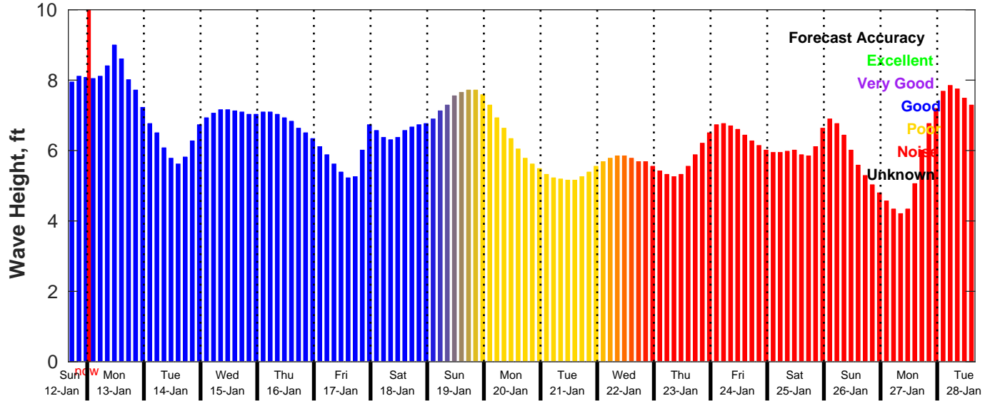
GFS Wave Forecast for NDBC 46028 from 12-Jan-2025 16:00:00 to 28-Jan-2025 16:00:00
