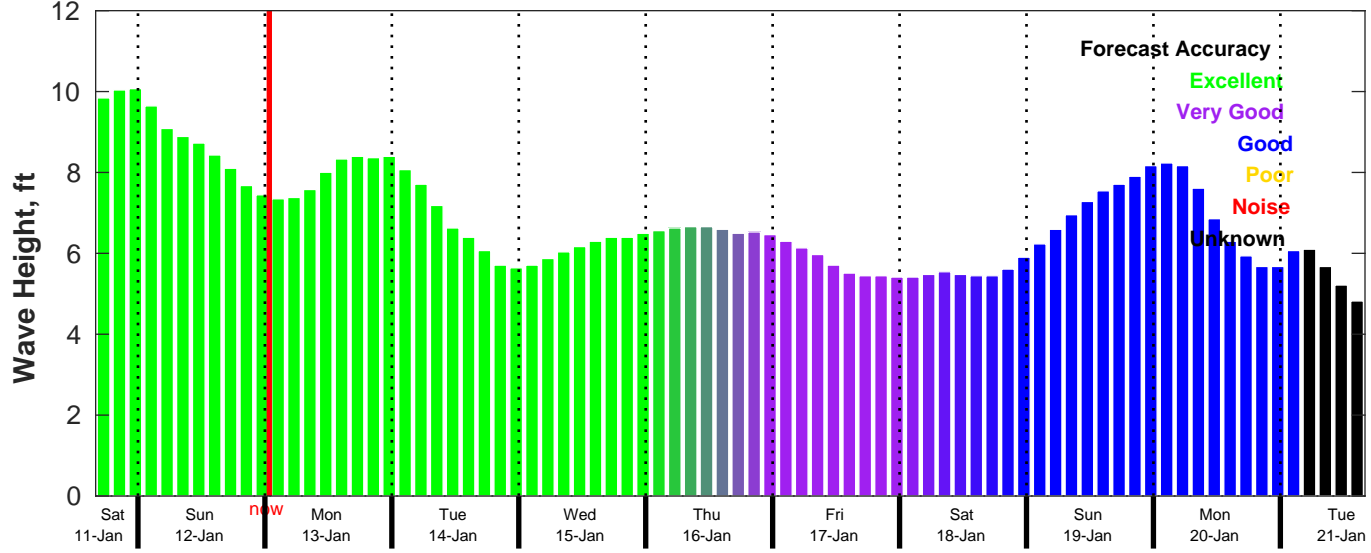
CMEMS Wave Forecast for NDBC 46069 from 11-Jan-2025 16:00:00 to 21-Jan-2025 16:00:00
