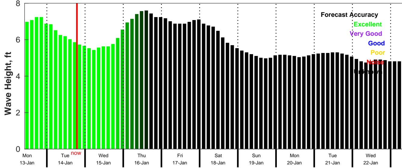
CMEMS Wave Forecast for NDBC 52211 from 12-Jan-2025 10:00:00 to 22-Jan-2025 10:00:00
