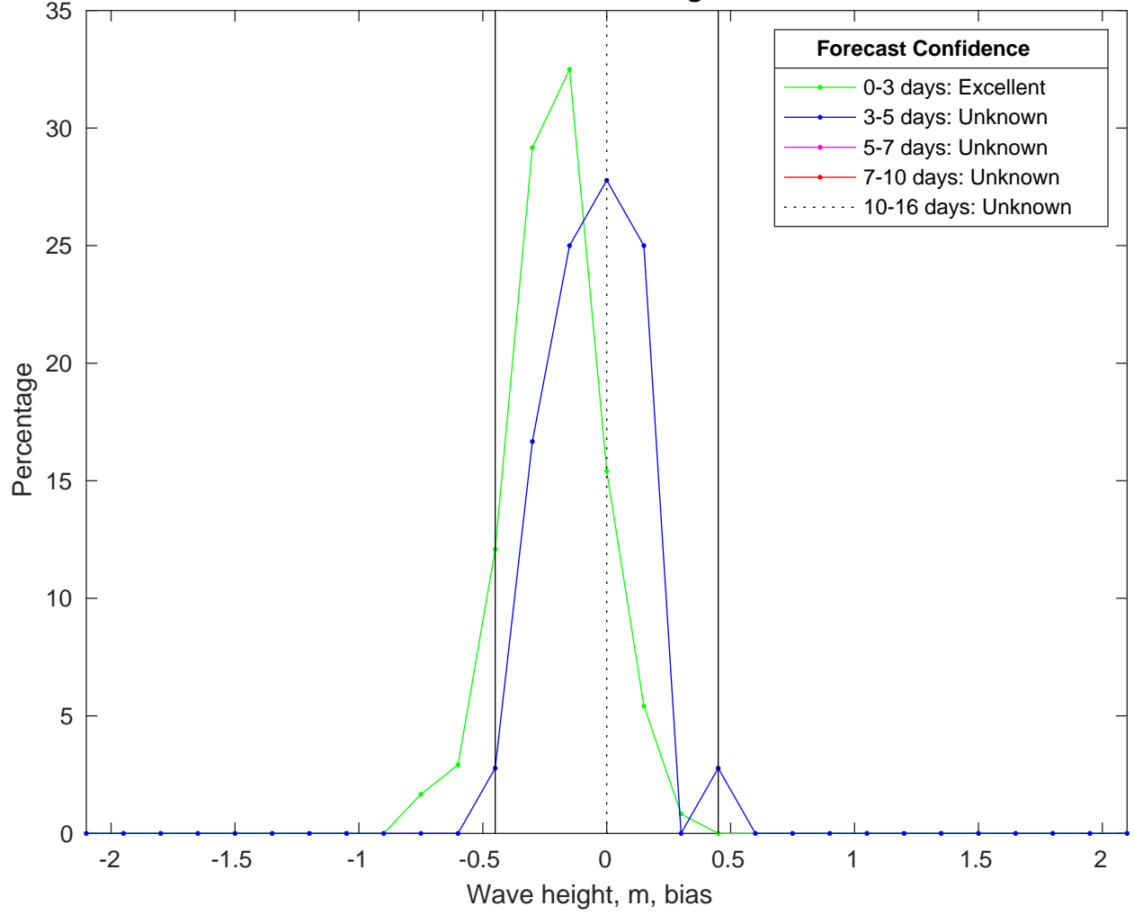
NDBC 52213 vs CMEMSWaves Bias Histogram: 13-Jan-2025
