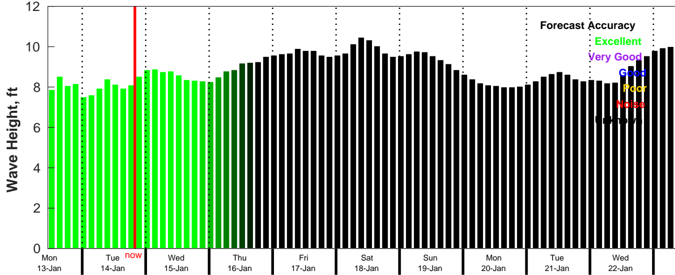
CMEMS Wave Forecast for NDBC 52213 from 12-Jan-2025 11:00:00 to 22-Jan-2025 11:00:00
