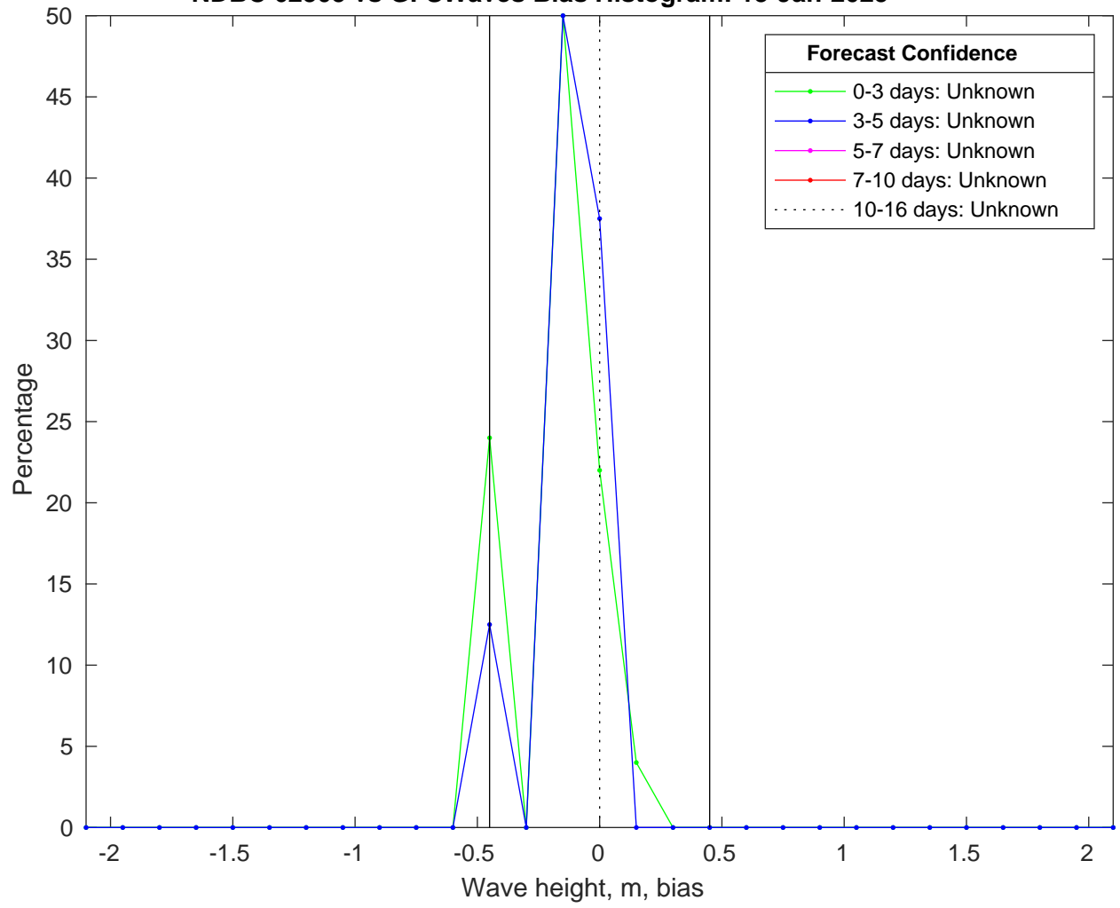
NDBC 62305 vs GFSWaves Bias Histogram: 13-Jan-2025
