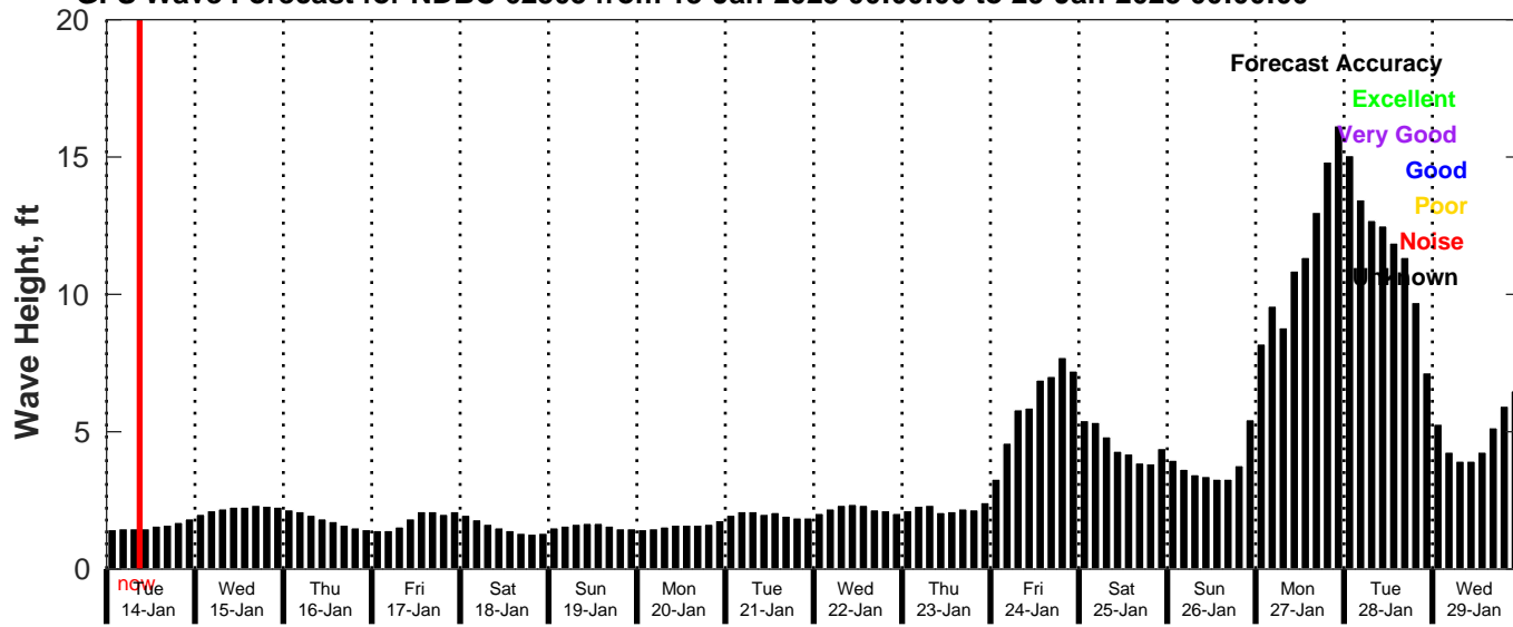
GFS Wave Forecast for NDBC 62305 from 13-Jan-2025 00:00:00 to 29-Jan-2025 00:00:00
