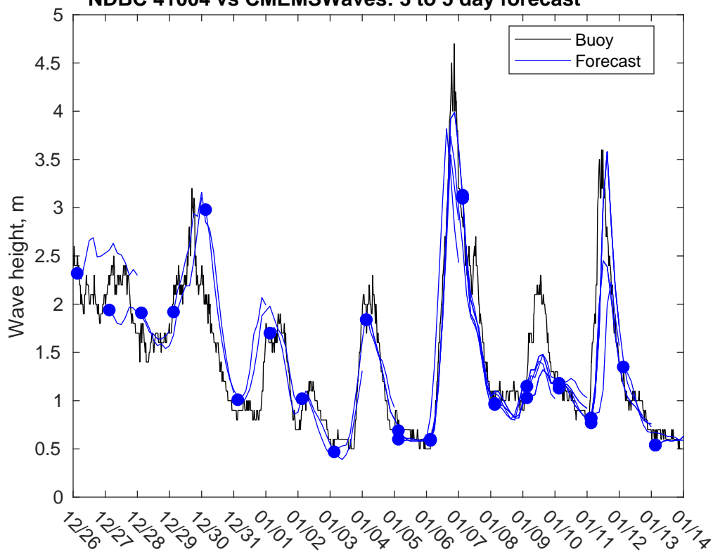
NDBC 41004 vs CMEMSWaves: 3 to 5 day forecast
