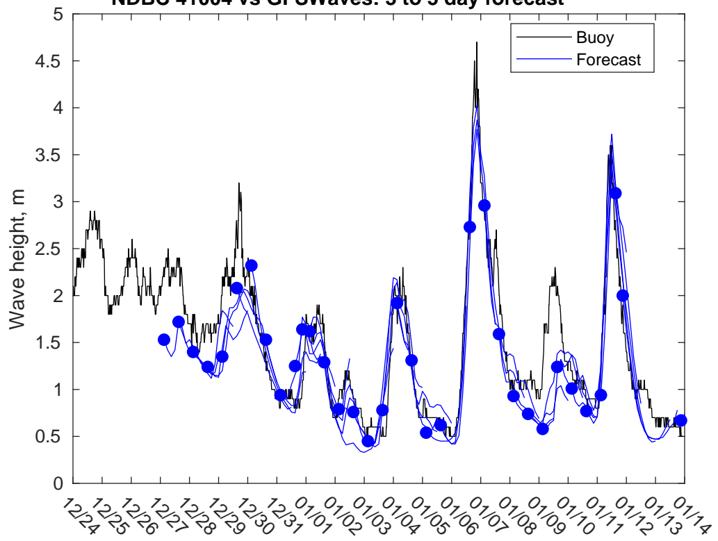
NDBC 41004 vs GFSWaves: 3 to 5 day forecast
