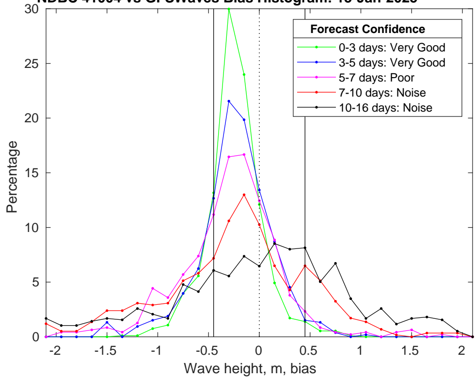
NDBC 41004 vs GFSWaves Bias Histogram: 13-Jan-2025
