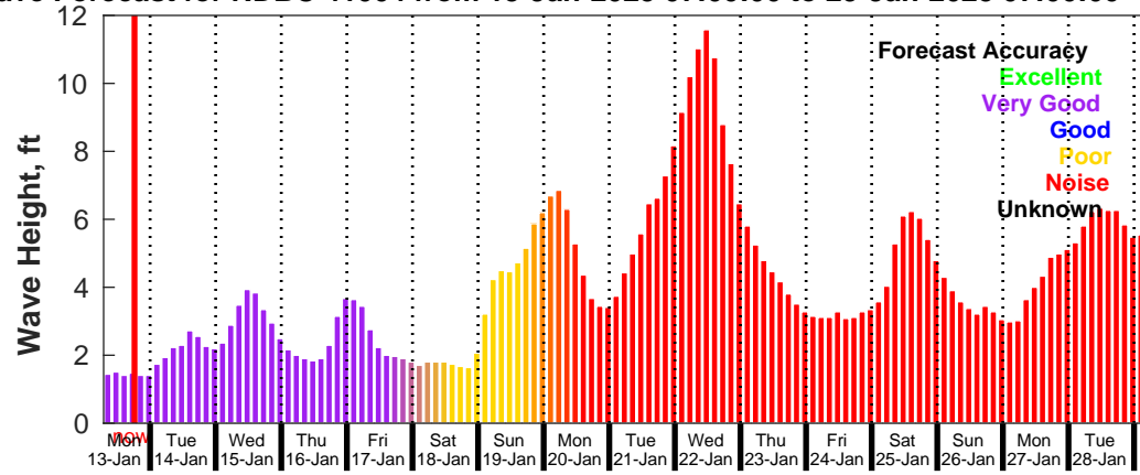
GFS Wave Forecast for NDBC 41004 from 13-Jan-2025 07:00:00 to 29-Jan-2025 07:00:00
