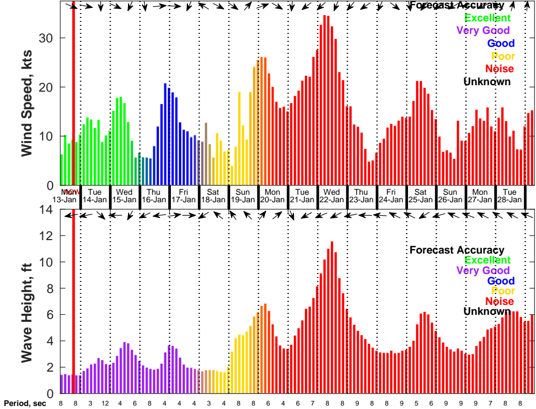
Wind & Wave Forecast for NDBC 41004 from 13-Jan-2025 07:00:00 to 29-Jan-2025 07:00:00
