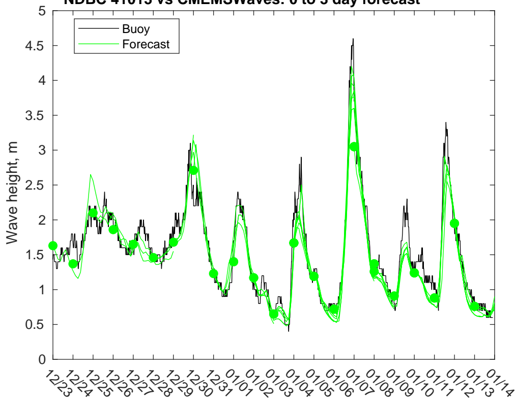
NDBC 41013 vs CMEMSWaves: 0 to 3 day forecast
