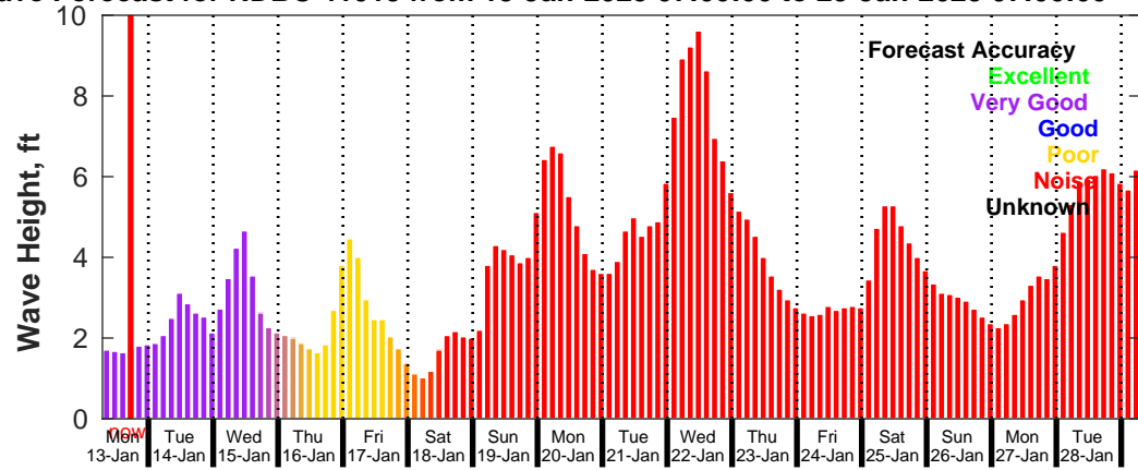
GFS Wave Forecast for NDBC 41013 from 13-Jan-2025 07:00:00 to 29-Jan-2025 07:00:00
