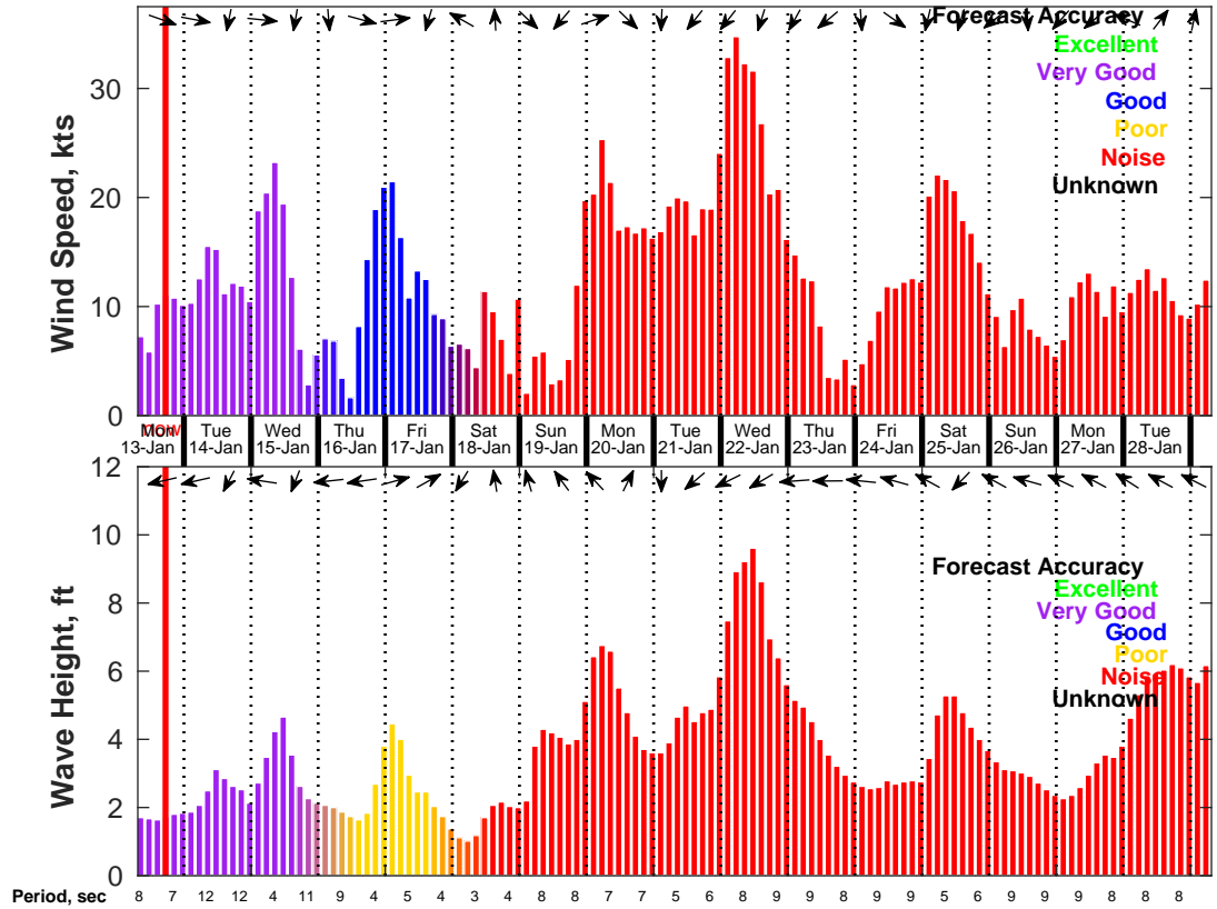
Wind & Wave Forecast for NDBC 41013 from 13-Jan-2025 07:00:00 to 29-Jan-2025 07:00:00
