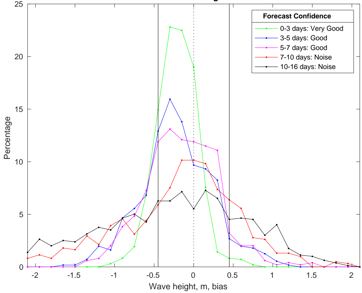
NDBC 42019 vs GFSWaves Bias Histogram: 13-Jan-2025
