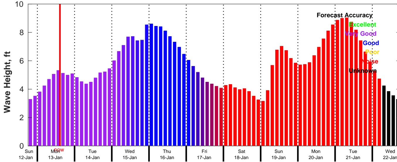
CMEMS Wave Forecast for NDBC 42019 from 12-Jan-2025 18:00:00 to 22-Jan-2025 18:00:00
