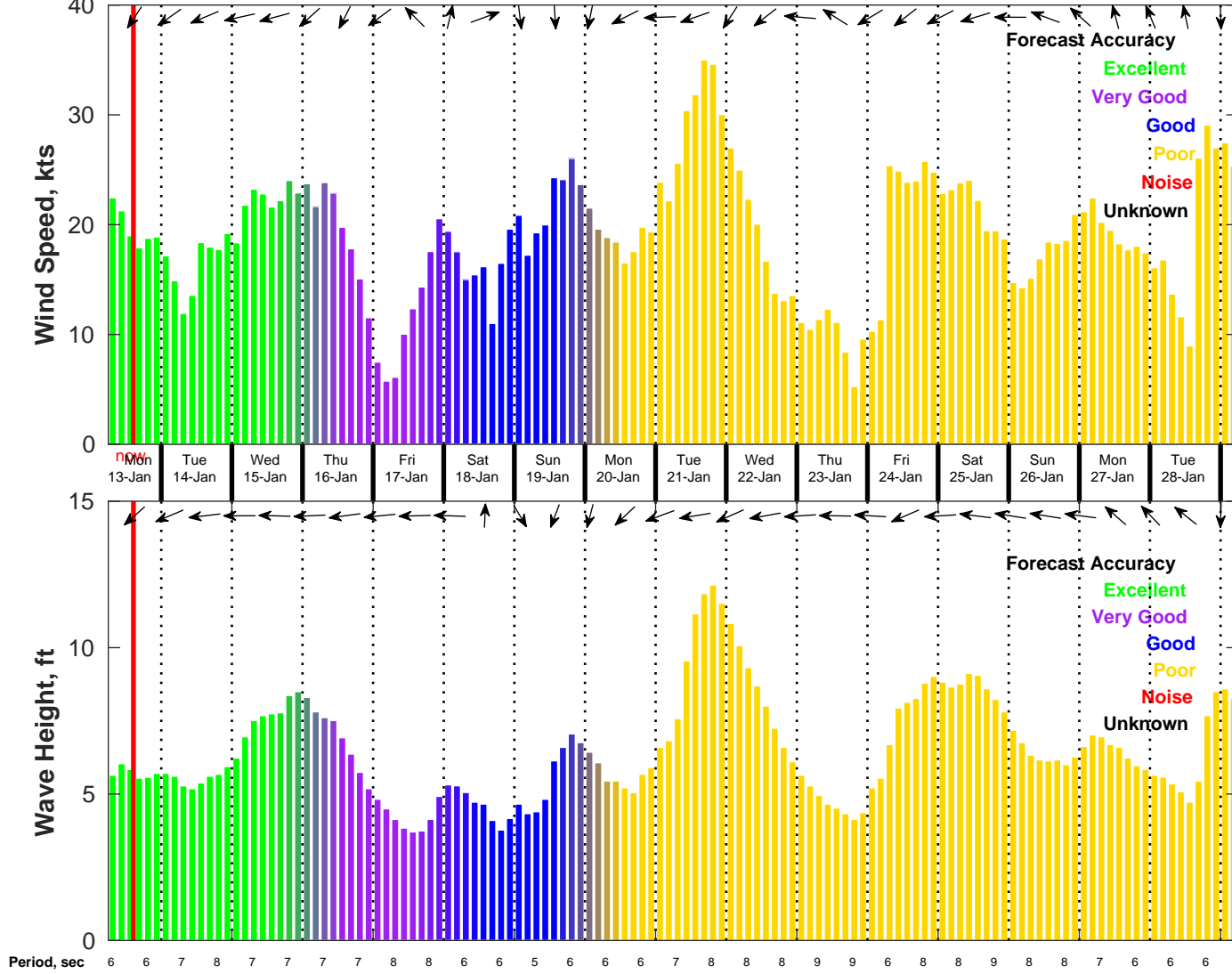
Wind & Wave Forecast for NDBC 42019 from 13-Jan-2025 06:00:00 to 29-Jan-2025 06:00:00
