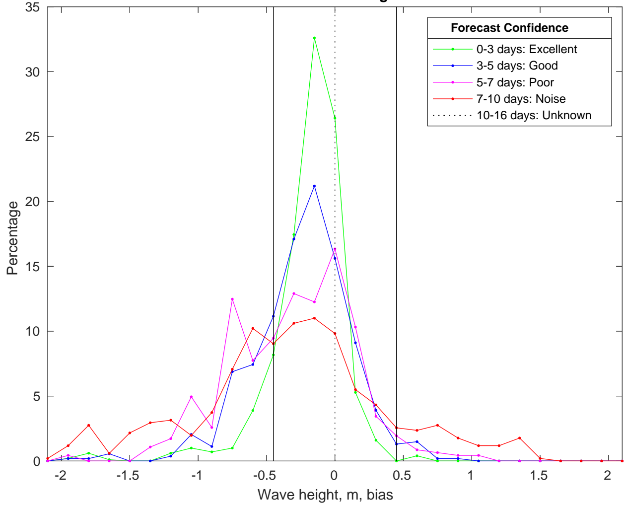
NDBC 42020 vs CMEMSWaves Bias Histogram: 13-Jan-2025
