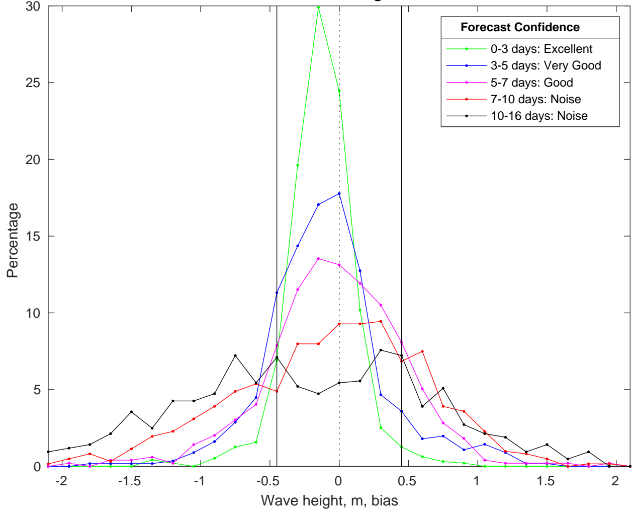
NDBC 42020 vs GFSWaves Bias Histogram: 13-Jan-2025
