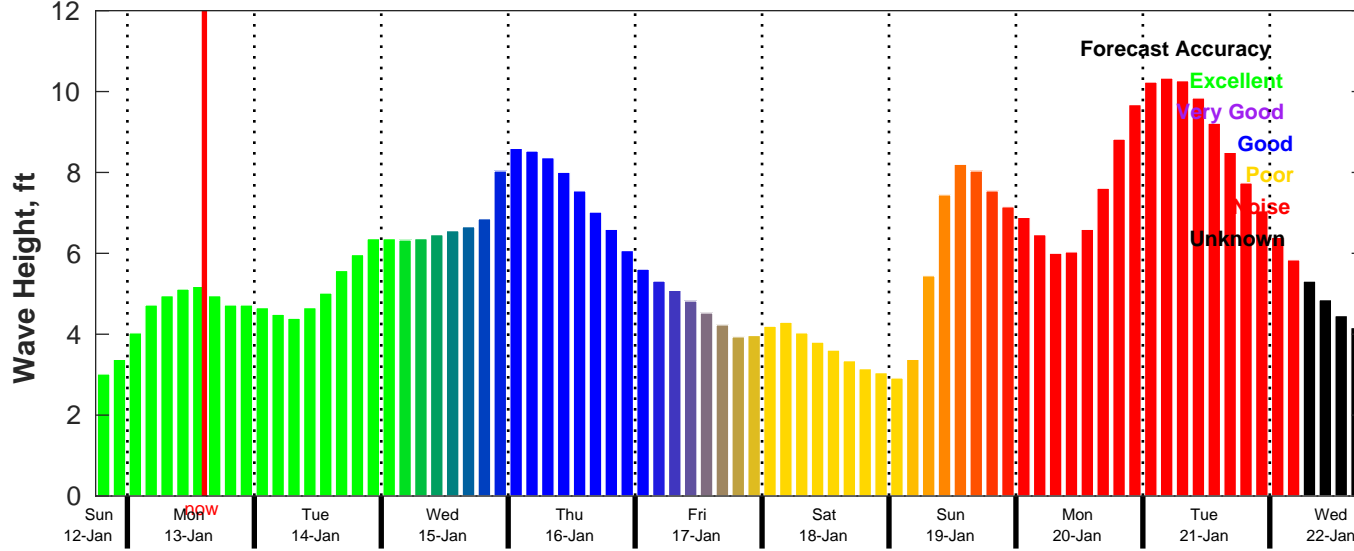
CMEMS Wave Forecast for NDBC 42020 from 12-Jan-2025 18:00:00 to 22-Jan-2025 18:00:00
