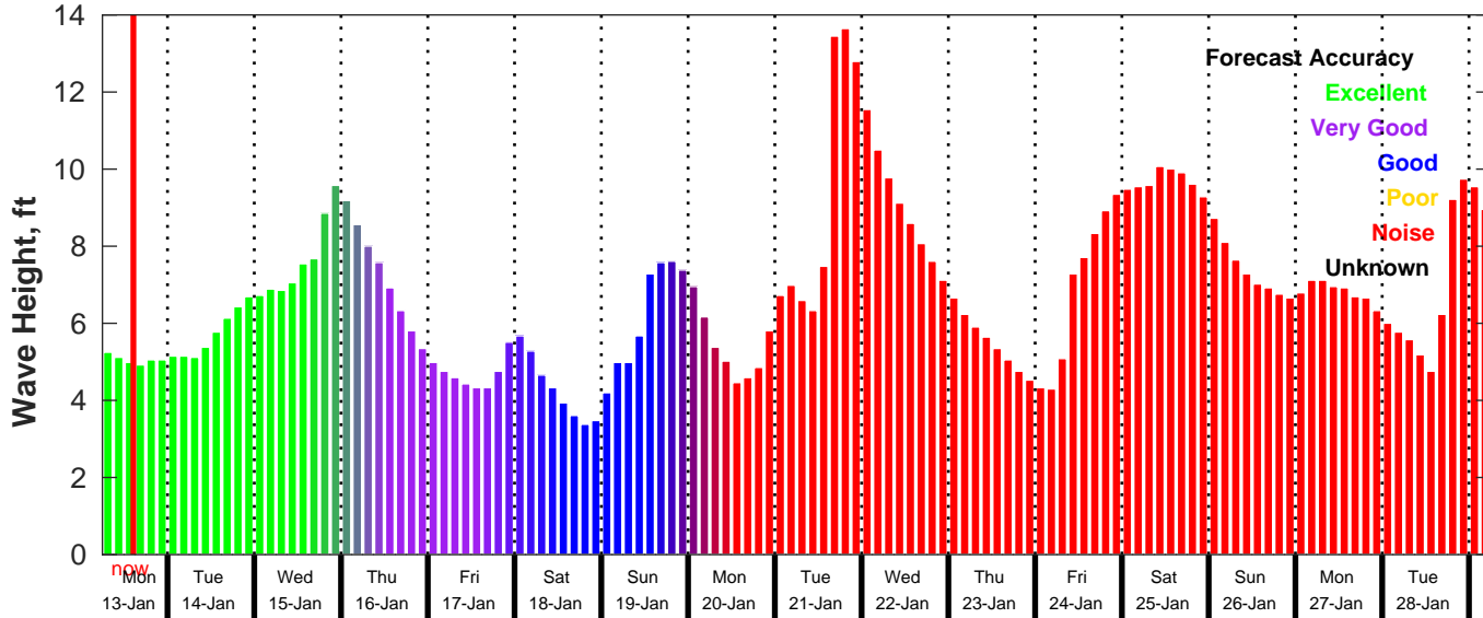
GFS Wave Forecast for NDBC 42020 from 13-Jan-2025 06:00:00 to 29-Jan-2025 06:00:00
