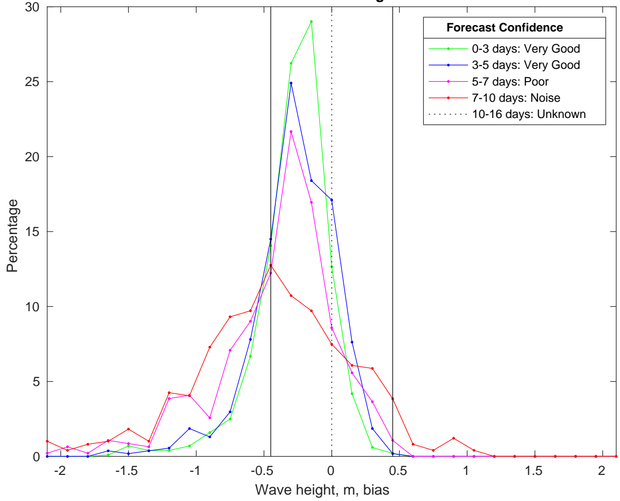
NDBC 42035 vs CMEMSWaves Bias Histogram: 13-Jan-2025
