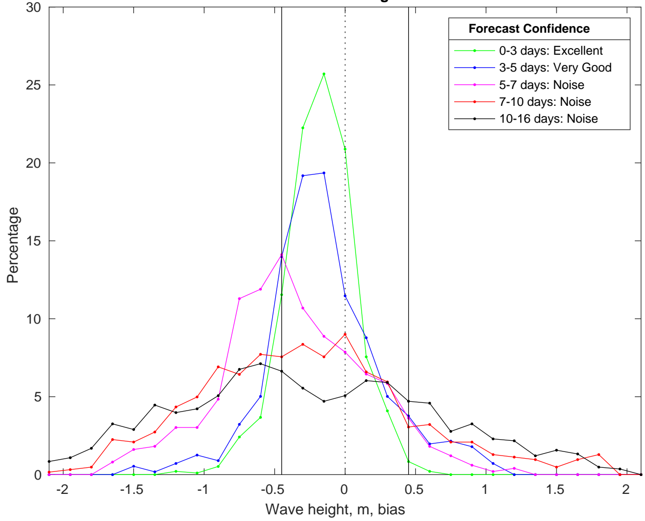
NDBC 42036 vs GFSWaves Bias Histogram: 13-Jan-2025
