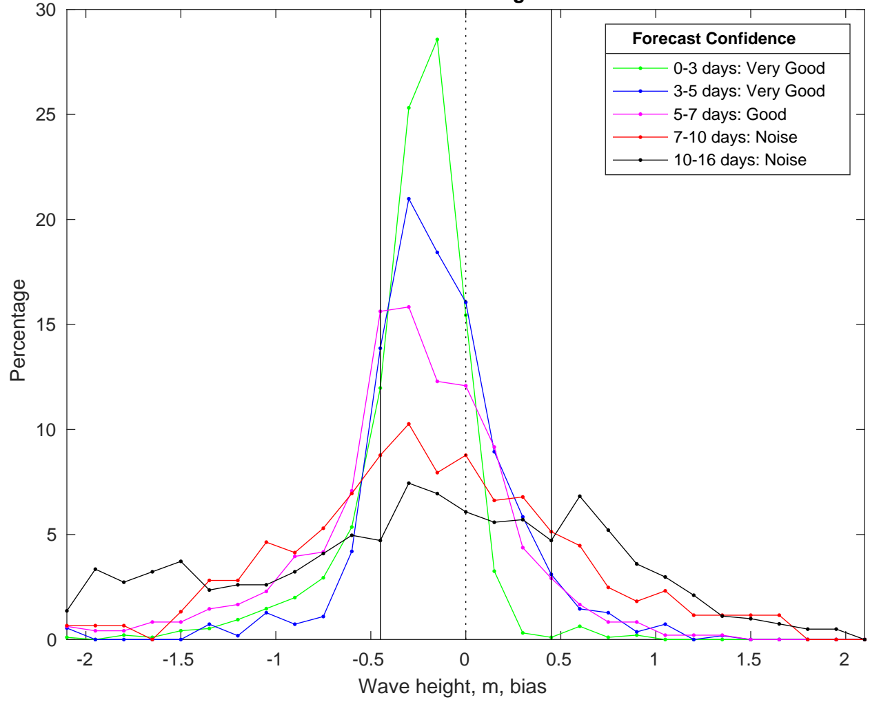
NDBC 42040 vs GFSWaves Bias Histogram: 13-Jan-2025
