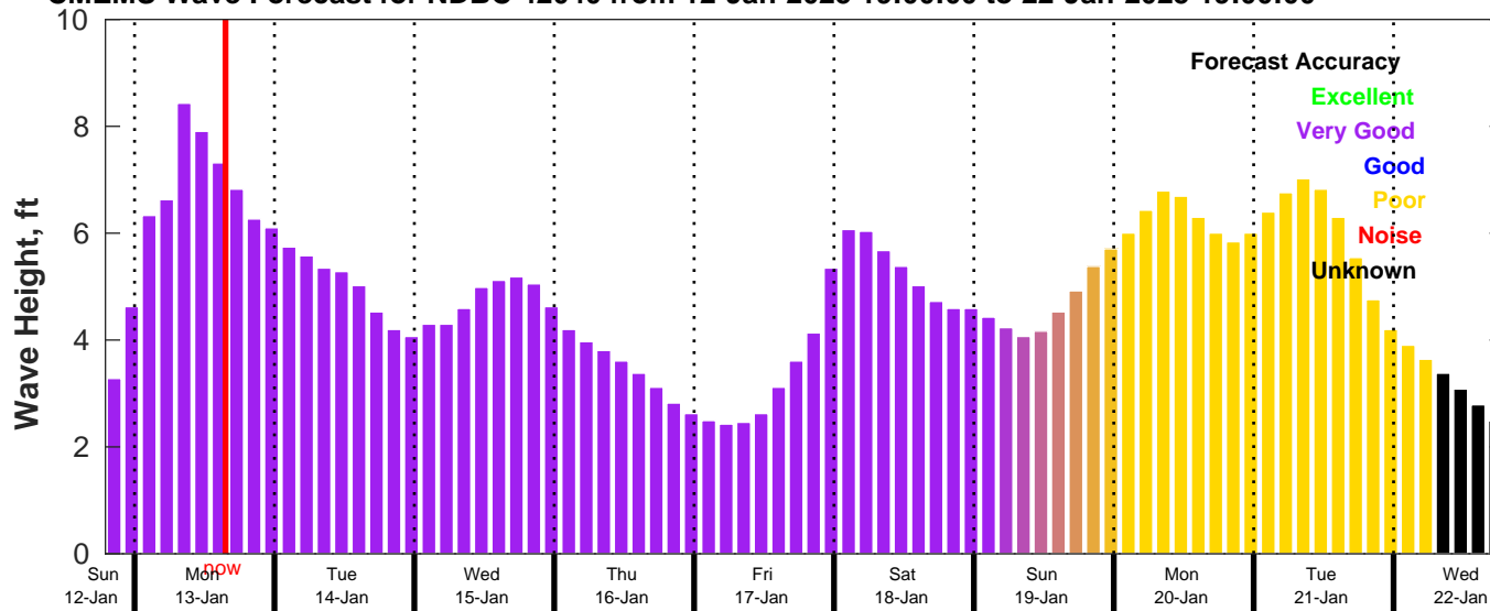
CMEMS Wave Forecast for NDBC 42040 from 12-Jan-2025 19:00:00 to 22-Jan-2025 19:00:00
