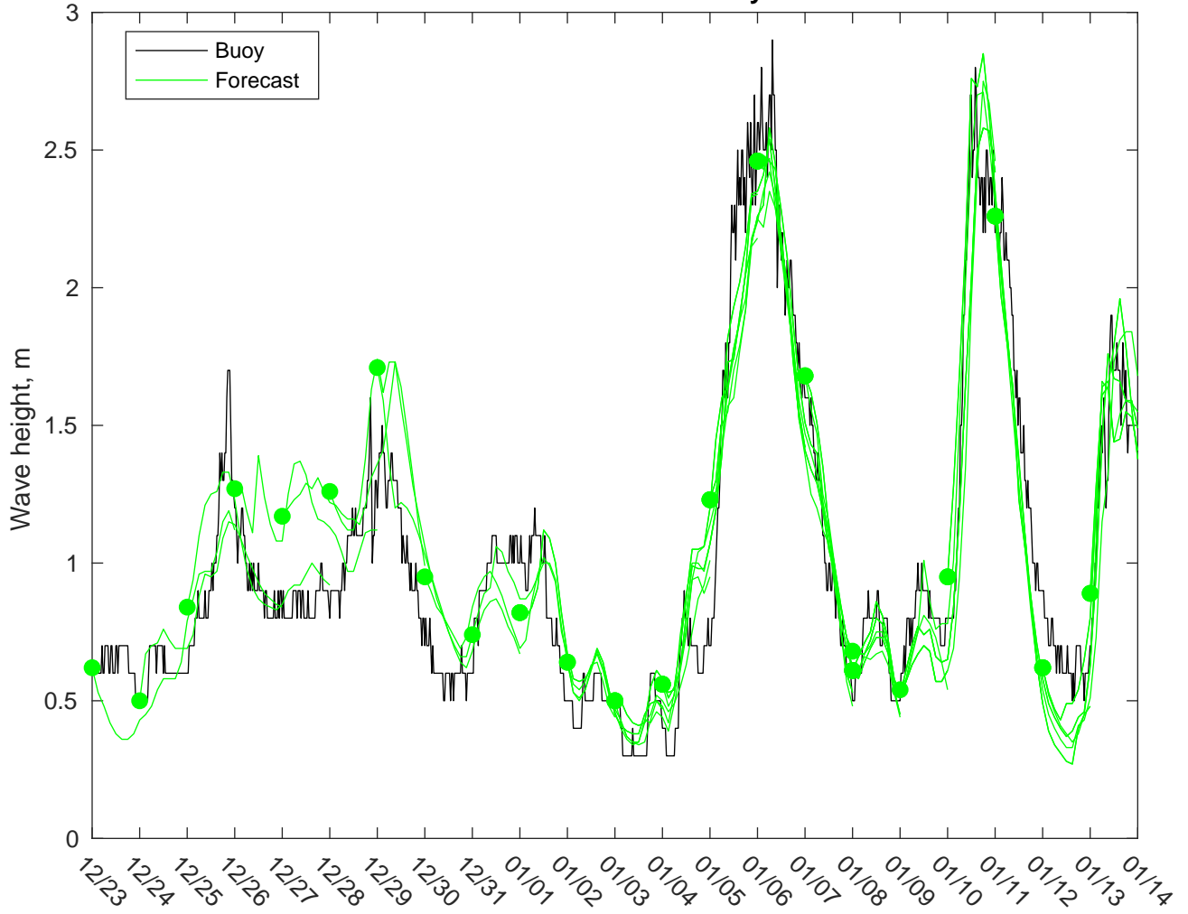
NDBC 42084 vs CMEMSWaves: 0 to 3 day forecast
