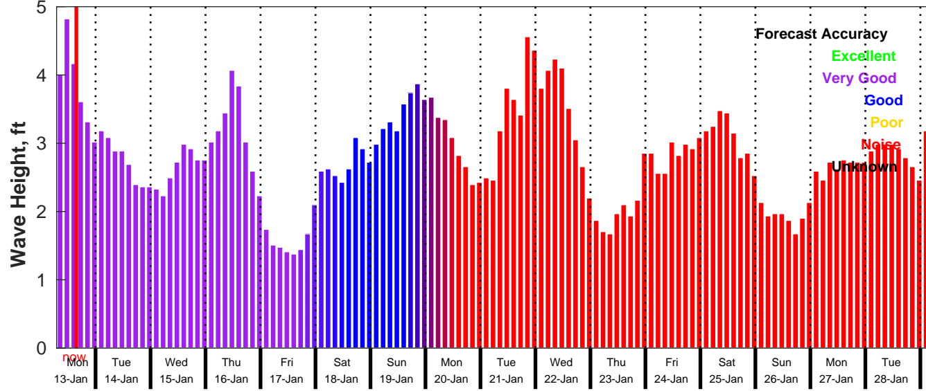
GFS Wave Forecast for NDBC 42084 from 13-Jan-2025 07:00:00 to 29-Jan-2025 07:00:00
