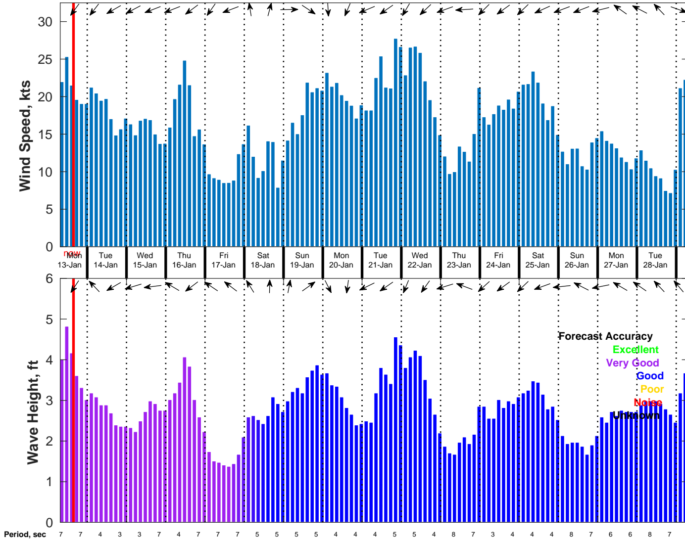
Wind & Wave Forecast for NDBC 42084 from 13-Jan-2025 07:00:00 to 29-Jan-2025 07:00:00
