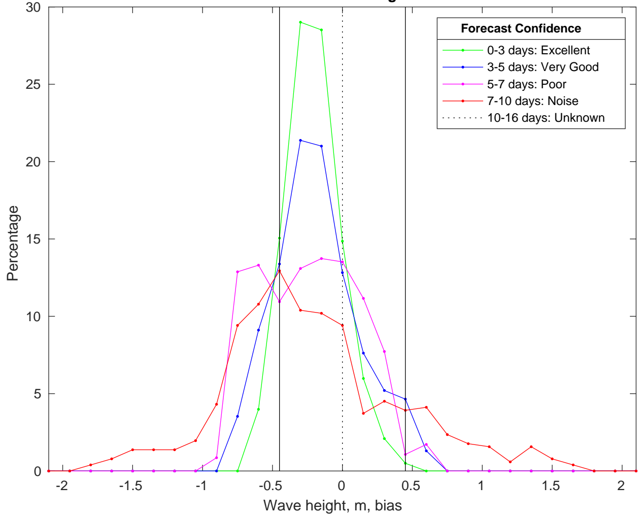
NDBC 42092 vs CMEMSWaves Bias Histogram: 13-Jan-2025
