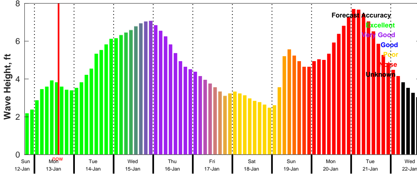
CMEMS Wave Forecast for NDBC 42092 from 12-Jan-2025 18:00:00 to 22-Jan-2025 18:00:00
