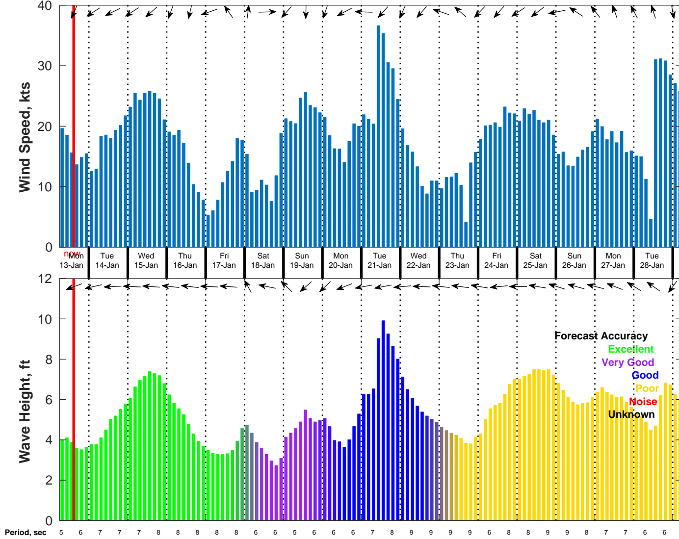
Wind & Wave Forecast for NDBC 42092 from 13-Jan-2025 06:00:00 to 29-Jan-2025 06:00:00
