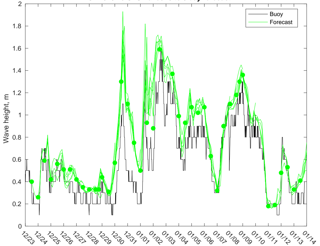
NDBC 44020 vs GFSWaves: 0 to 3 day forecast
