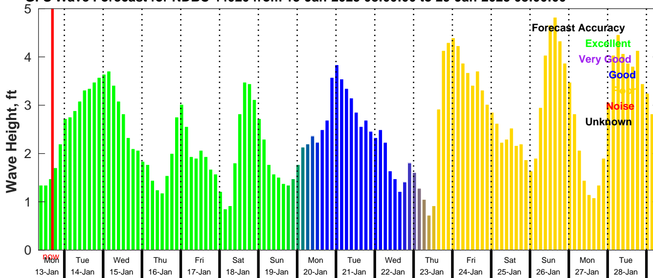
GFS Wave Forecast for NDBC 44020 from 13-Jan-2025 08:00:00 to 29-Jan-2025 08:00:00
