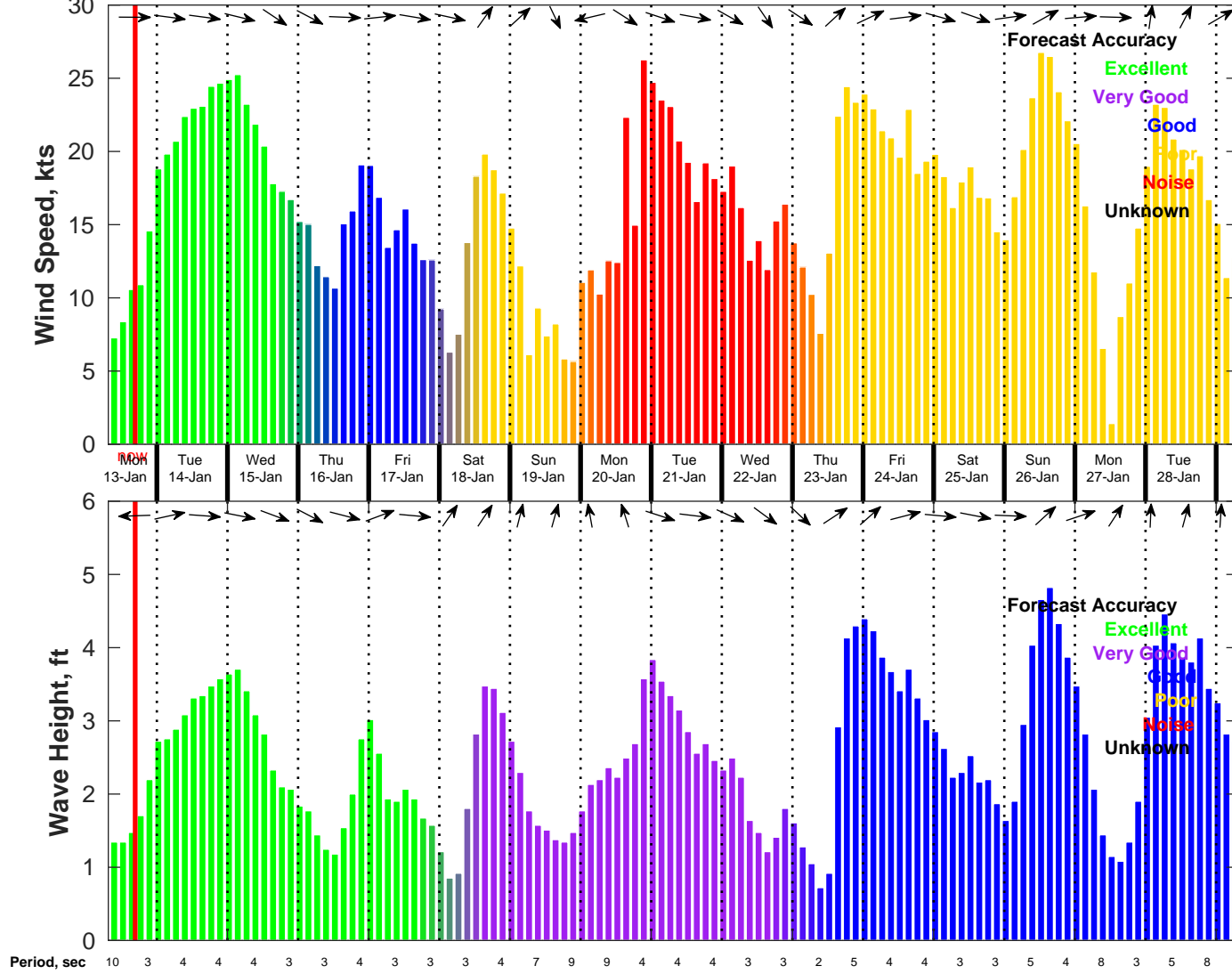
Wind & Wave Forecast for NDBC 44020 from 13-Jan-2025 08:00:00 to 29-Jan-2025 08:00:00
