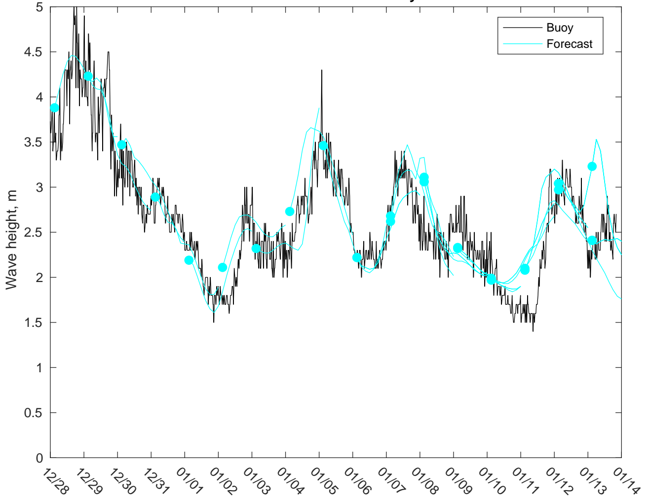
NDBC 46011 vs CMEMSWaves: 5 to 7 day forecast
