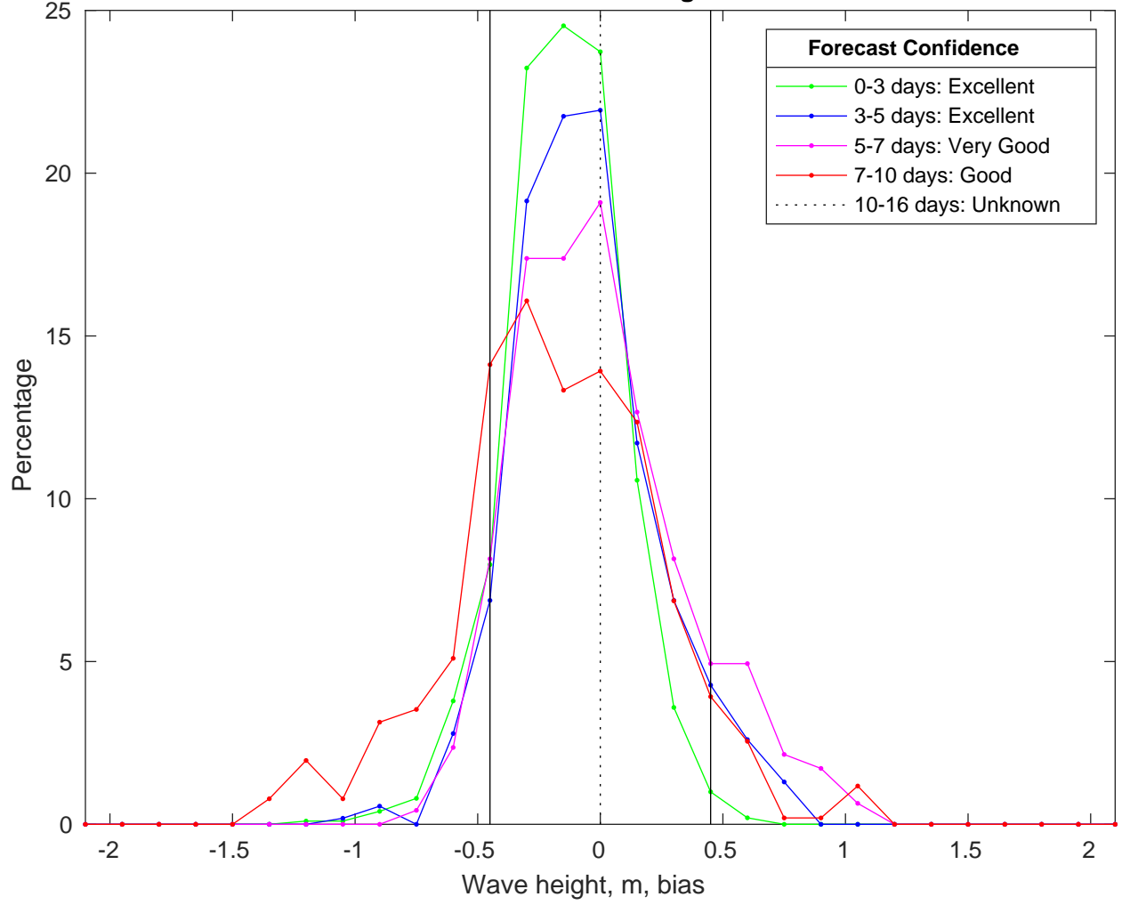
NDBC 46011 vs CMEMSWaves Bias Histogram: 13-Jan-2025
