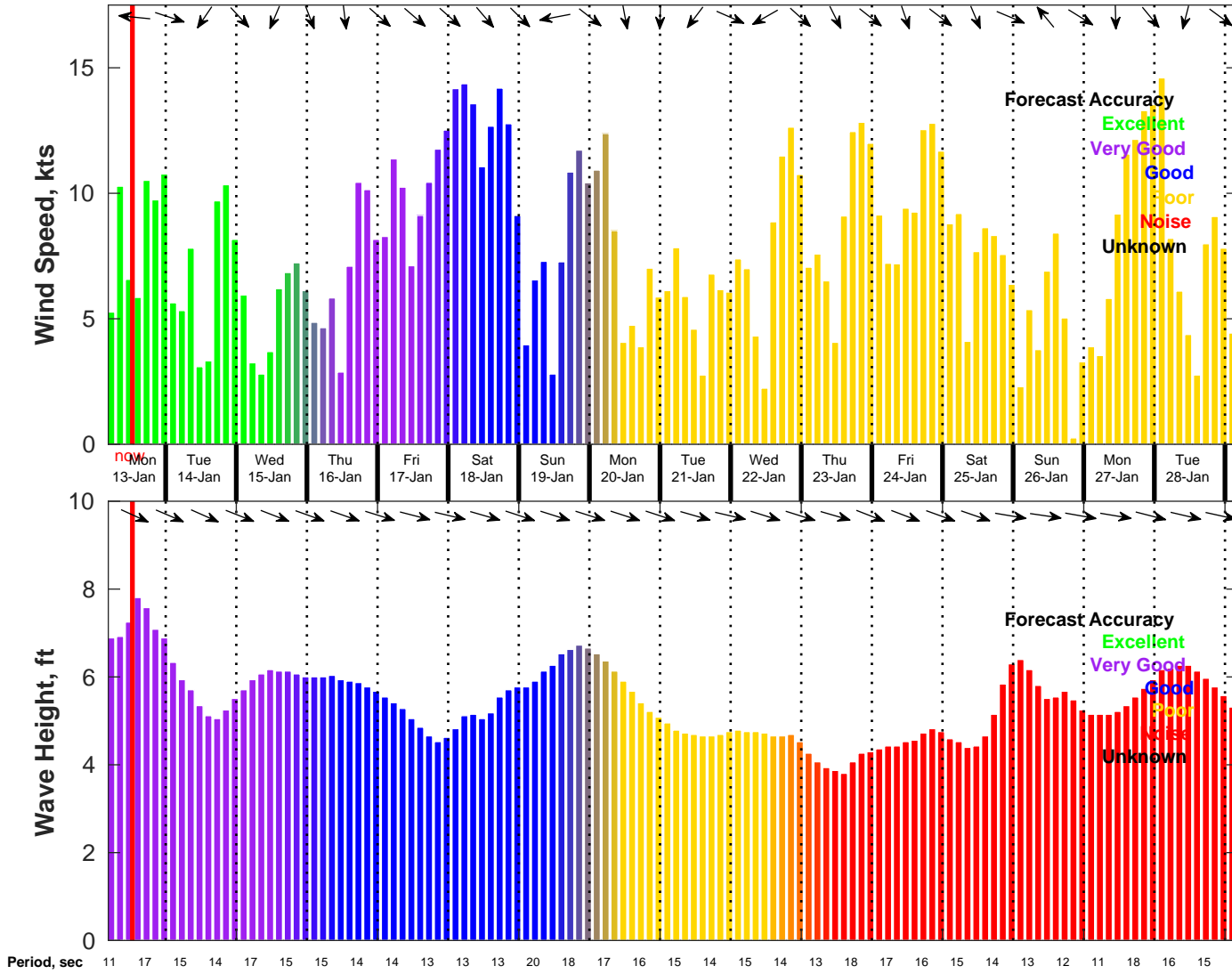
Wind & Wave Forecast for NDBC 46011 from 13-Jan-2025 04:00:00 to 29-Jan-2025 04:00:00
