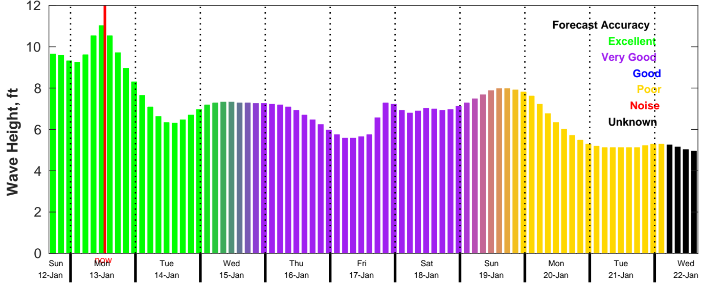
CMEMS Wave Forecast for NDBC 46028 from 12-Jan-2025 16:00:00 to 22-Jan-2025 16:00:00
