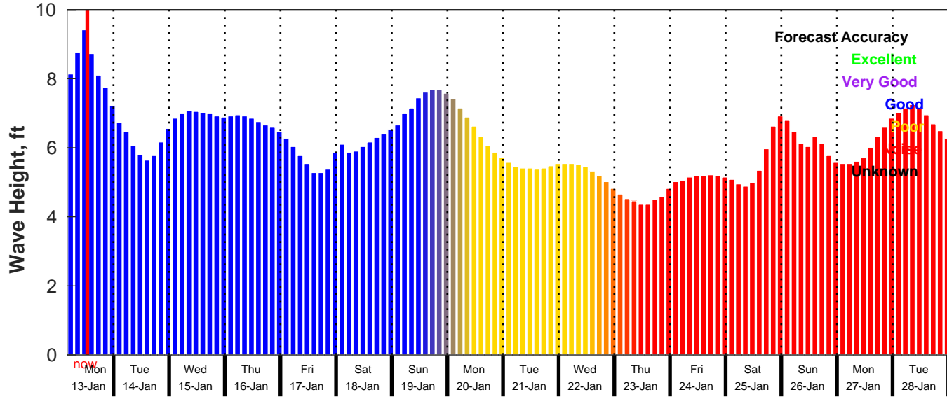
GFS Wave Forecast for NDBC 46028 from 13-Jan-2025 04:00:00 to 29-Jan-2025 04:00:00
