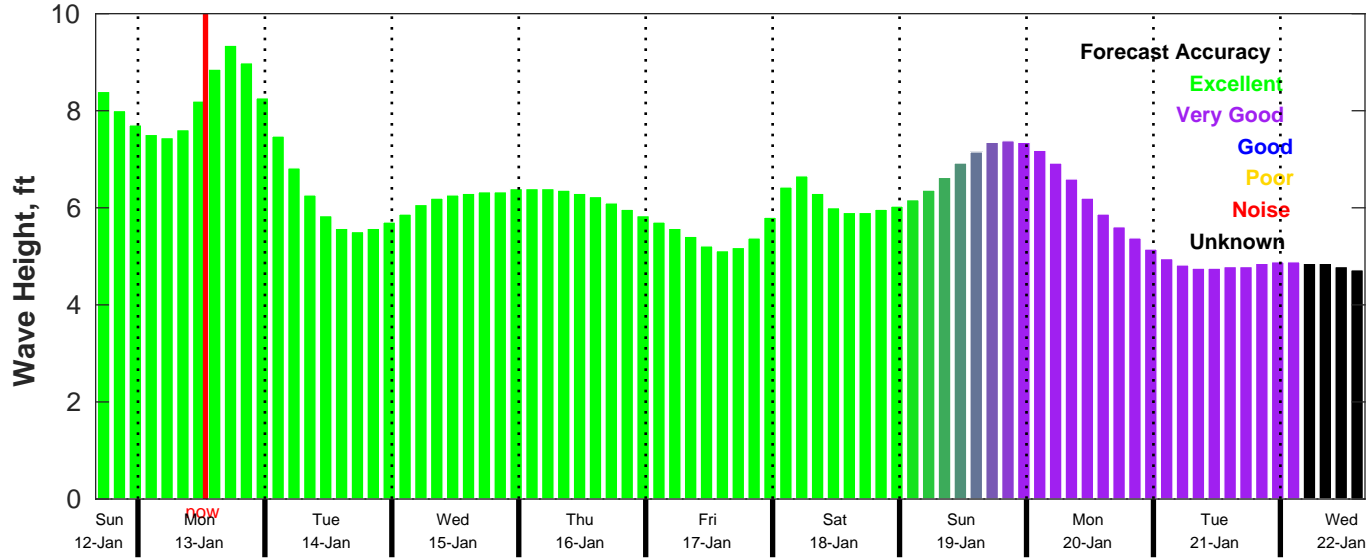
CMEMS Wave Forecast for NDBC 46054 from 12-Jan-2025 16:00:00 to 22-Jan-2025 16:00:00
