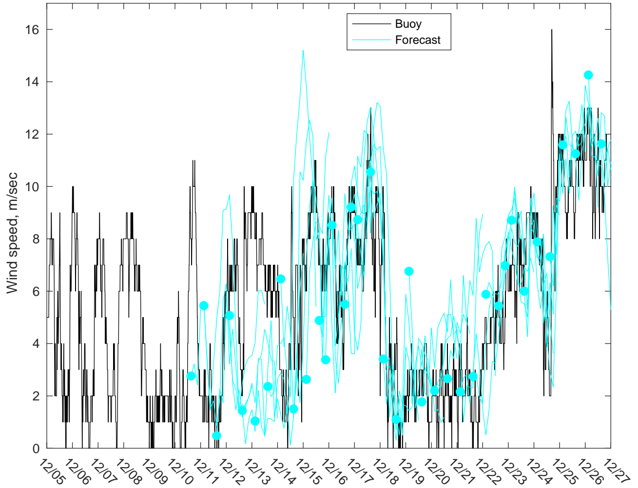
NDBC 46054 vs GFSWinds: 5 to 7 day forecast
