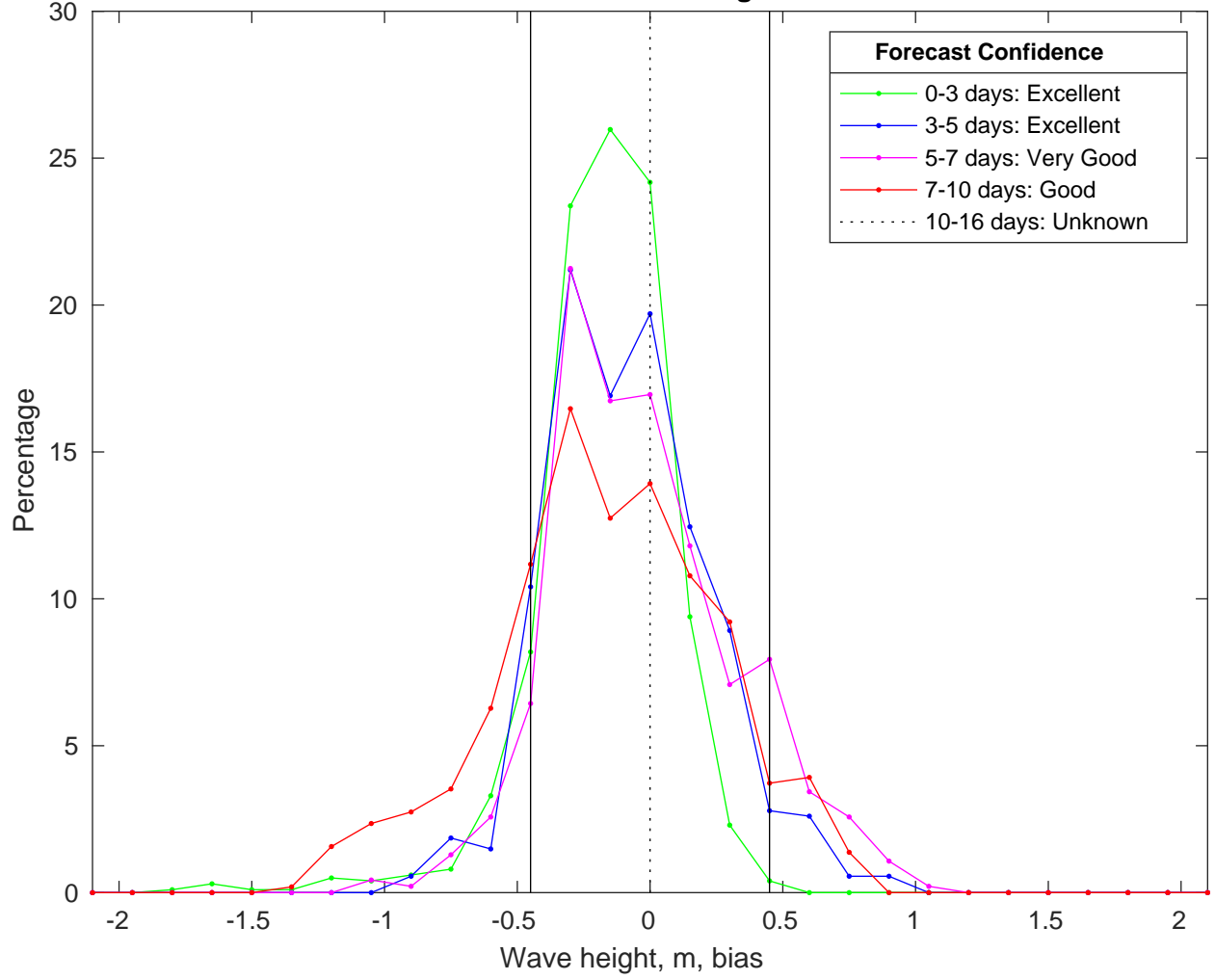
NDBC 46069 vs CMEMSWaves Bias Histogram: 13-Jan-2025
