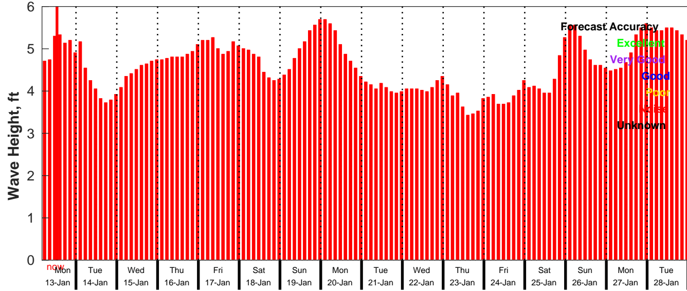
GFS Wave Forecast for NDBC 46069 from 13-Jan-2025 04:00:00 to 29-Jan-2025 04:00:00
