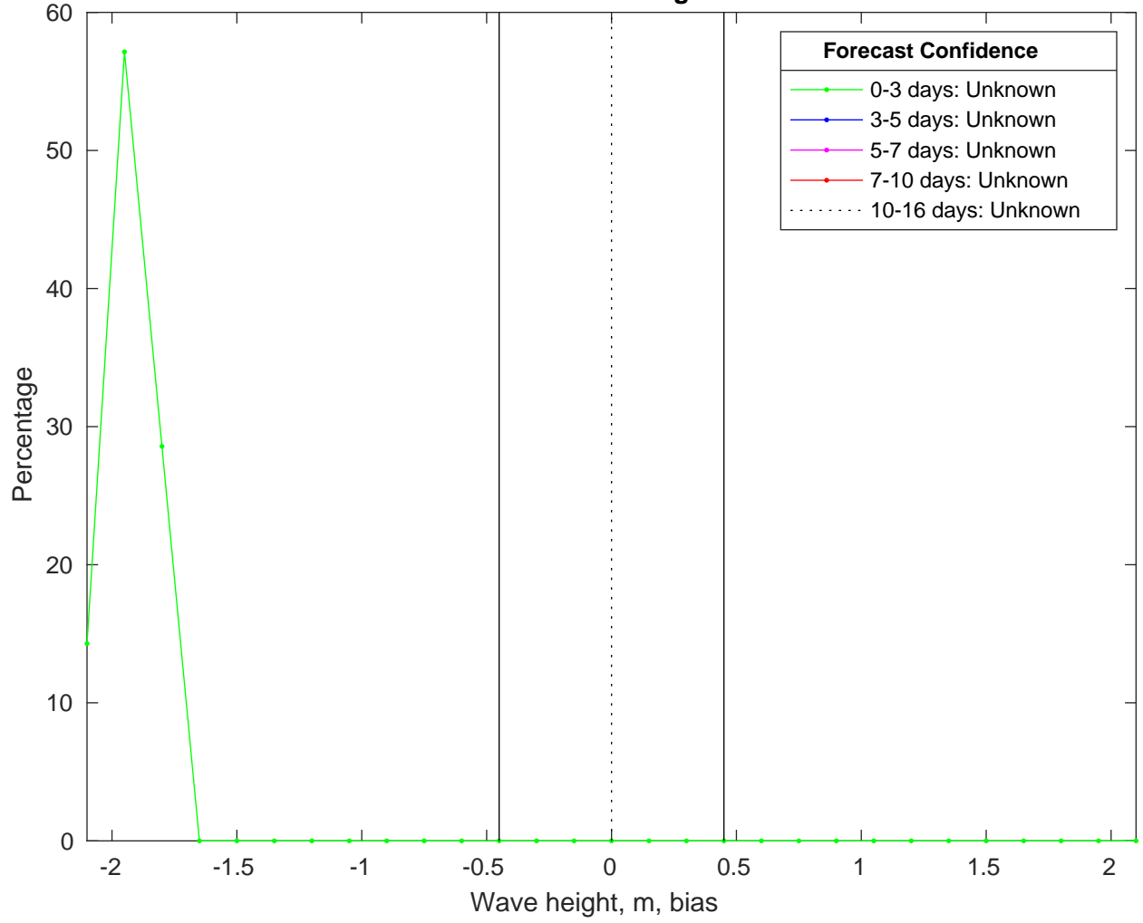
NDBC 46246 vs GFSWaves Bias Histogram: 13-Jan-2025
