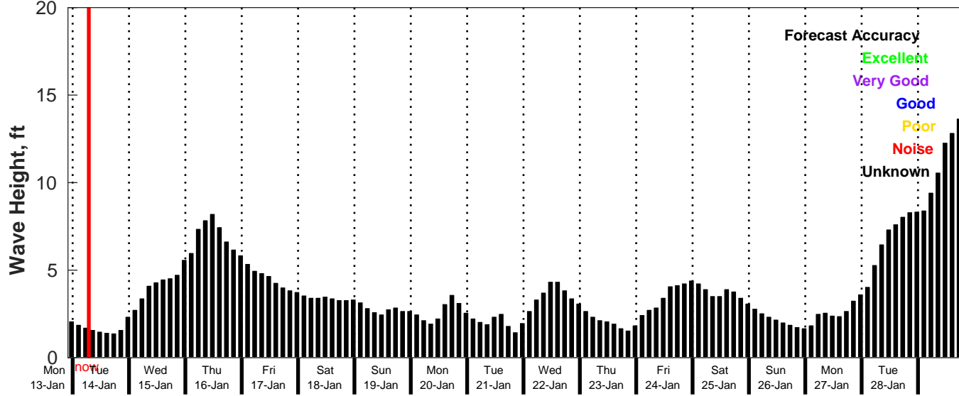
GFS Wave Forecast for NDBC 46246 from 13-Jan-2025 22:00:00 to 29-Jan-2025 22:00:00
