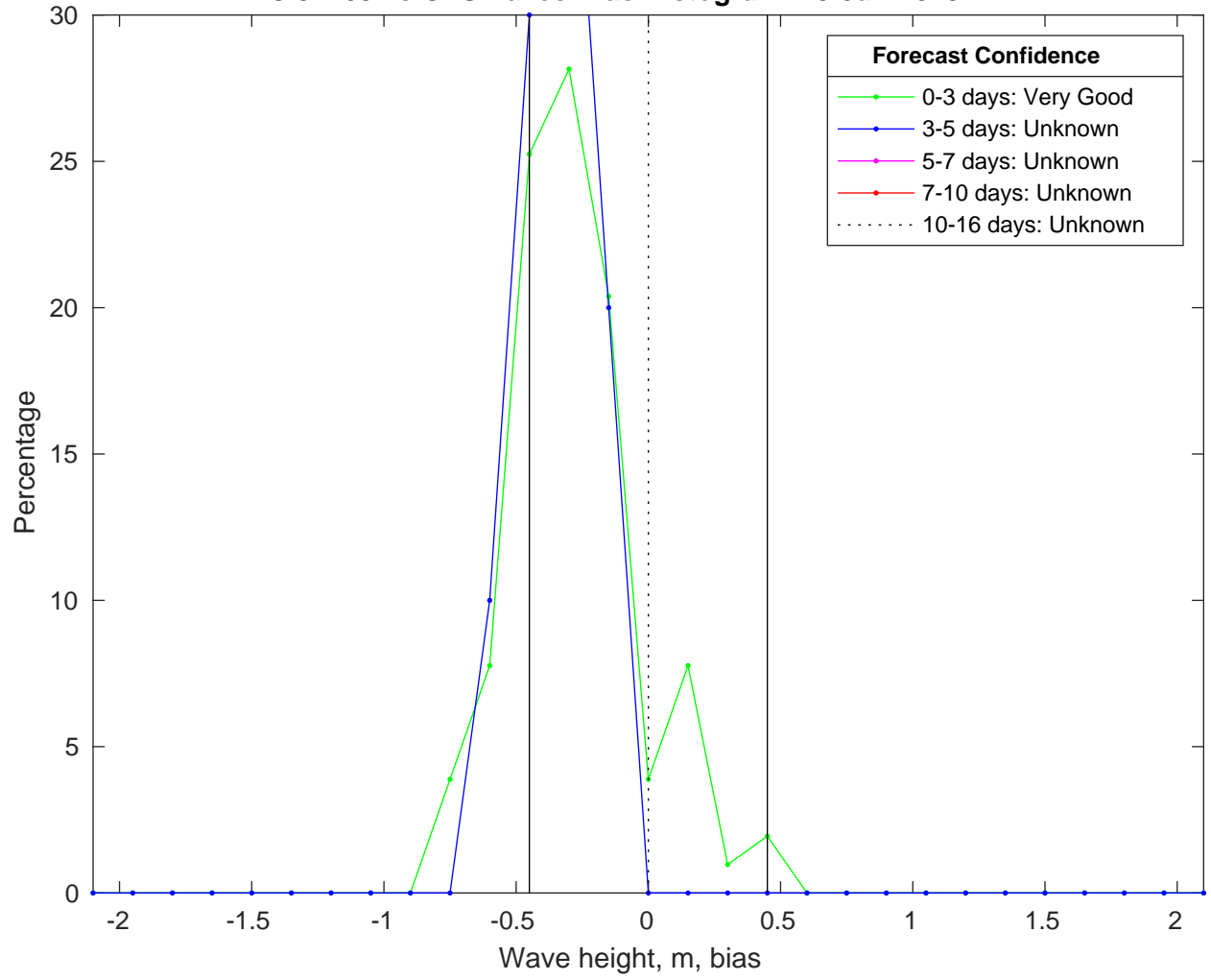
NDBC 51209 vs GFSWaves Bias Histogram: 13-Jan-2025
