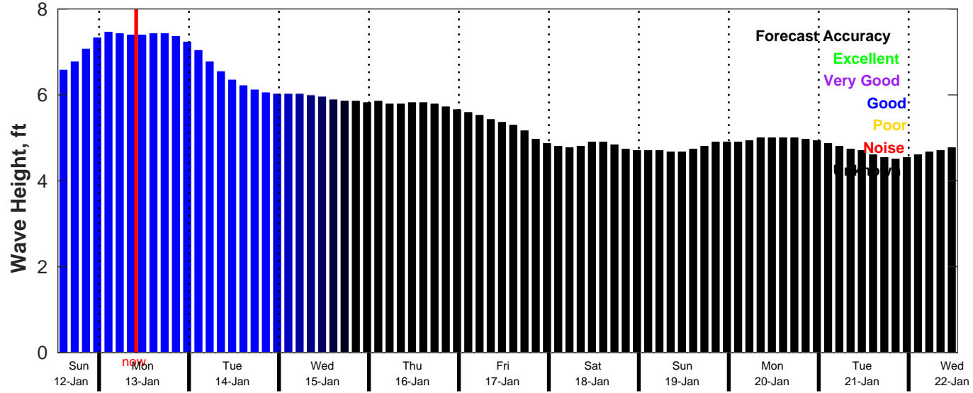
CMEMS Wave Forecast for NDBC 51209 from 12-Jan-2025 13:00:00 to 22-Jan-2025 13:00:00
